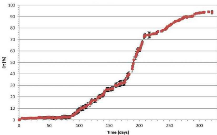
Figure 10. Evolution of the percentage of biodegradation (average value) of sample AST-21-097-05
